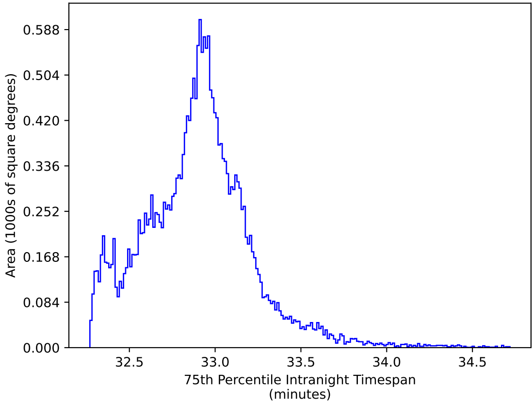
ddf_acor_sf10_lsf20_lsr20_v3.4_10yrs All sky y band: 75th Percentile Intranight Timespan
