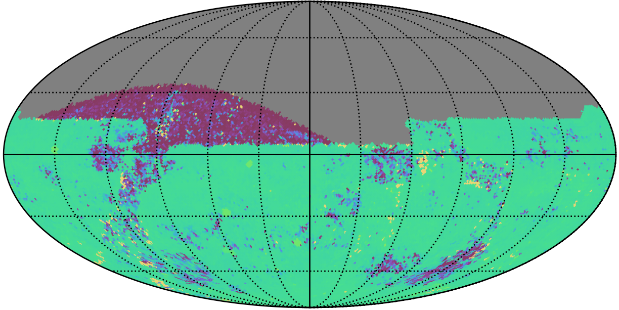
ddf_acor_sf10_lsf20_lsr20_v3.4_10yrs All sky ug bands: 75th Percentile Intranight Timespan
