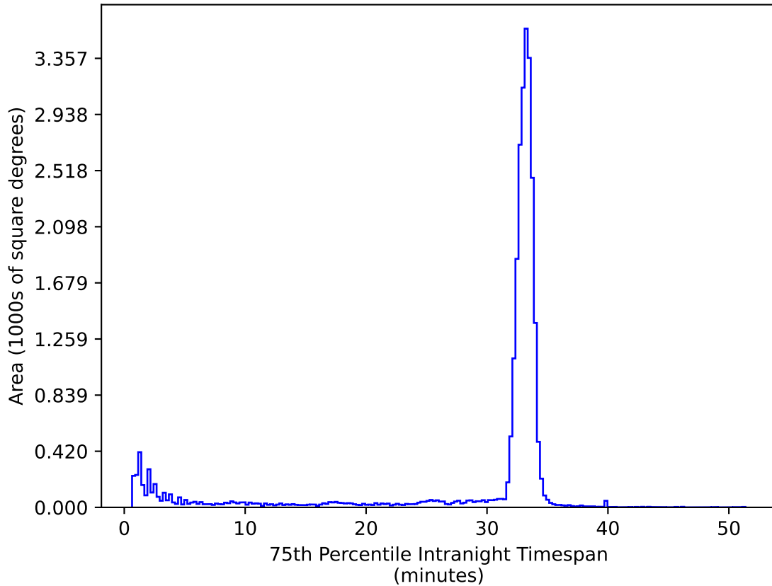
ddf_acor_sf10_lsf20_lsr20_v3.4_10yrs All sky ug bands: 75th Percentile Intranight Timespan
