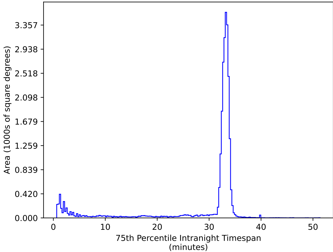
ddf_acor_sf10_lsf20_lsr20_v3.4_10yrs All sky ug bands: 75th Percentile Intranight Timespan
