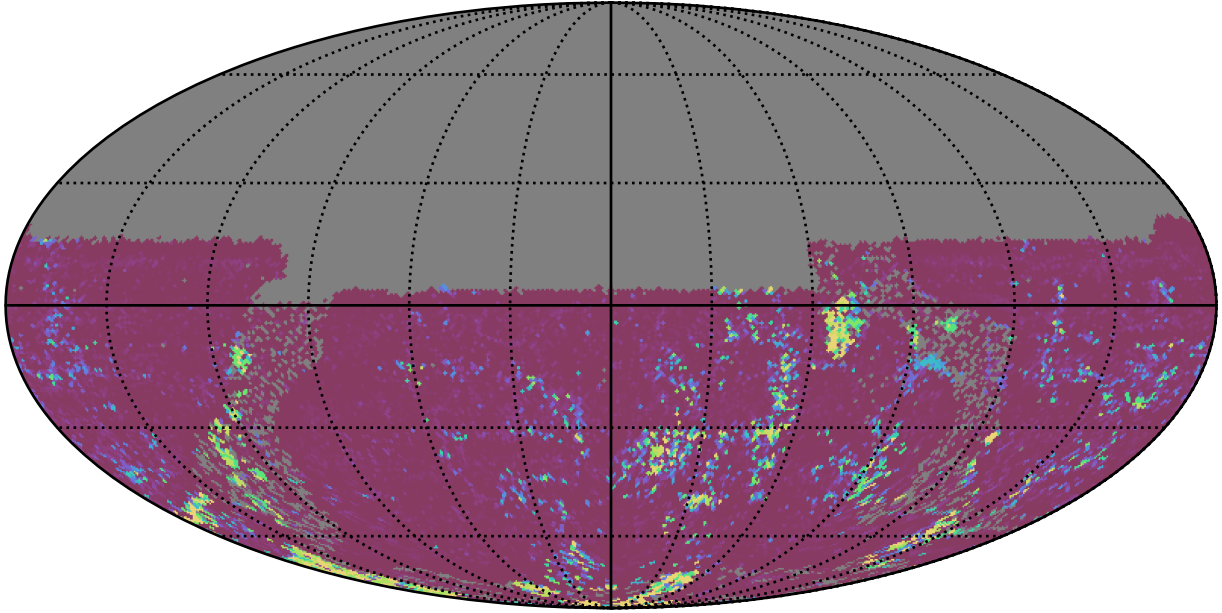
ddf_acor_sf10_lsf20_lsr20_v3.4_10yrs All sky u band: 75th Percentile Intranight Timespan
