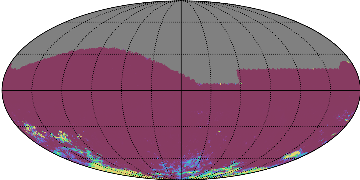
ddf_acor_sf10_lsf20_lsr20_v3.4_10yrs All sky ri bands: 75th Percentile Intranight Timespan
