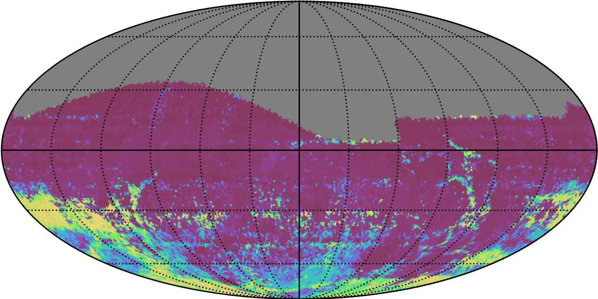
ddf_acor_sf10_lsf20_lsr20_v3.4_10yrs All sky r band: 75th Percentile Intranight Timespan
