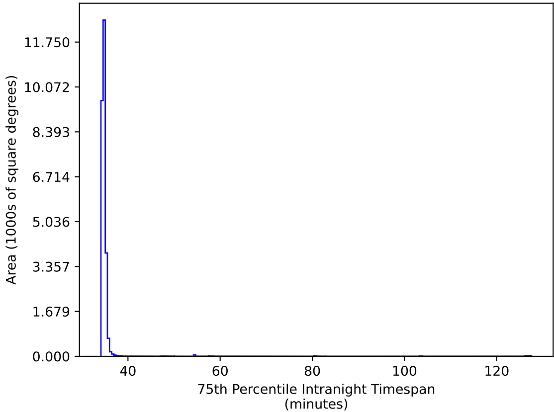
ddf_acor_sf10_lsf20_lsr20_v3.4_10yrs All sky iz bands: 75th Percentile Intranight Timespan
