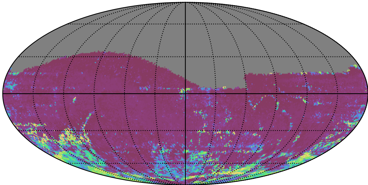
ddf_acor_sf10_lsf20_lsr20_v3.4_10yrs All sky i band: 75th Percentile Intranight Timespan
