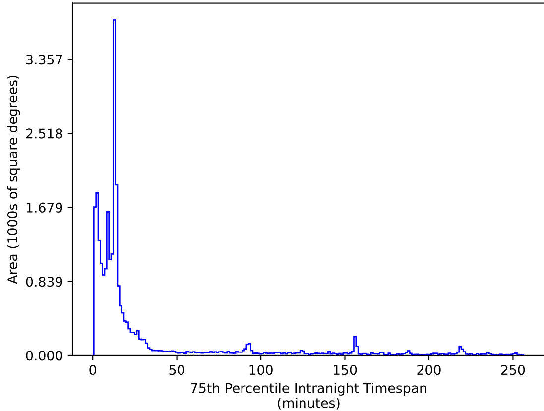
ddf_acor_sf10_lsf20_lsr20_v3.4_10yrs All sky i band: 75th Percentile Intranight Timespan
