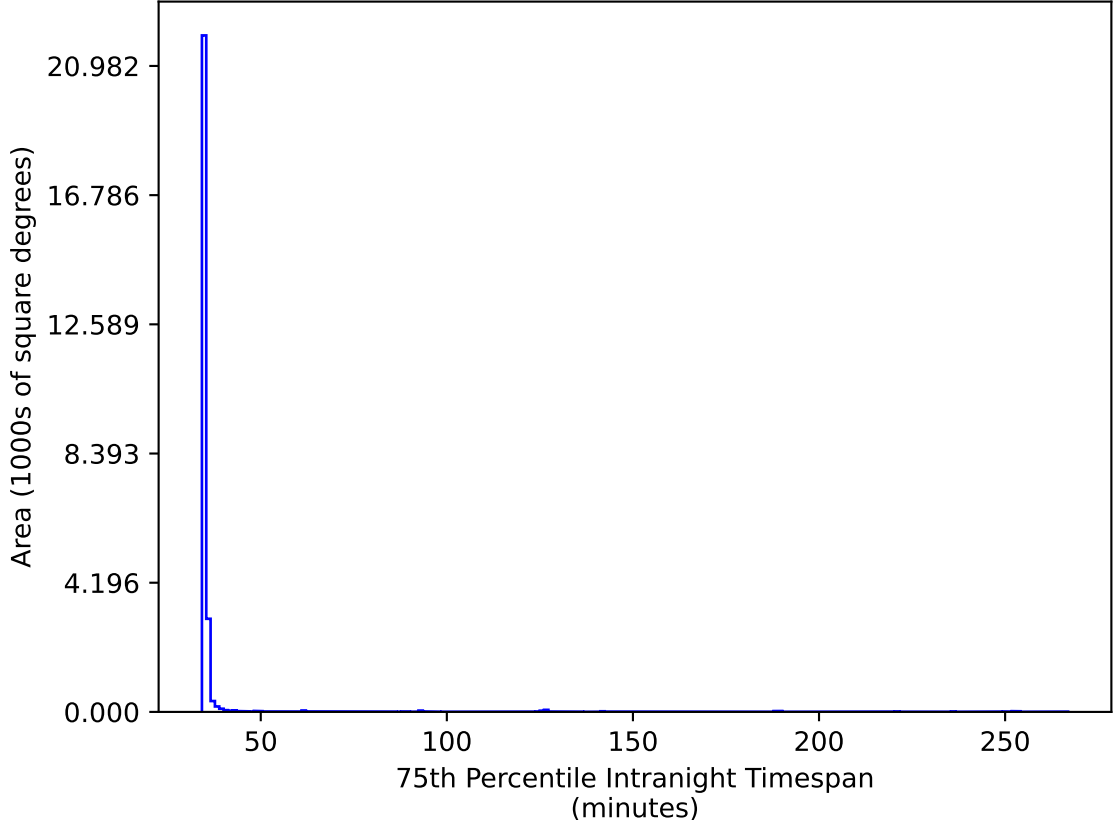
ddf_acor_sf10_lsf20_lsr20_v3.4_10yrs All sky gr bands: 75th Percentile Intranight Timespan
