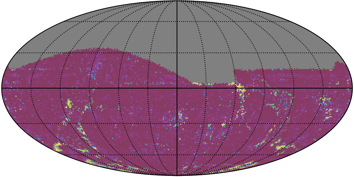
ddf_acor_sf10_lsf20_lsr20_v3.4_10yrs All sky g band: 75th Percentile Intranight Timespan
