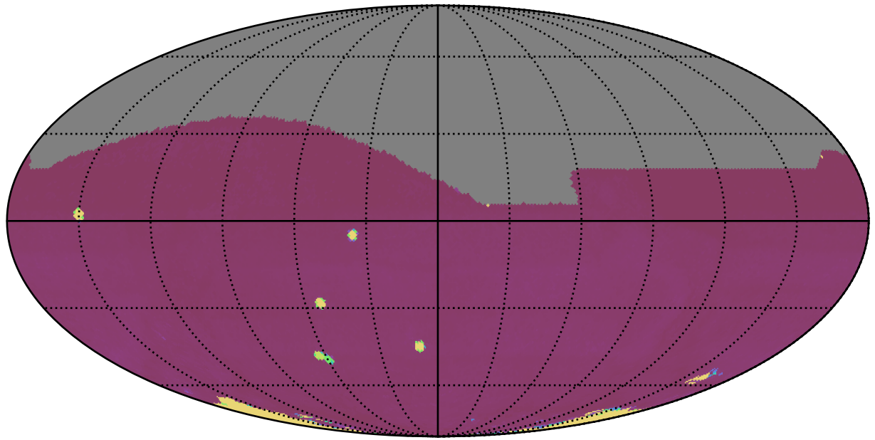
ddf_acor_sf10_lsf20_lsr20_v3.4_10yrs All sky: 75th Percentile Intranight Timespan
