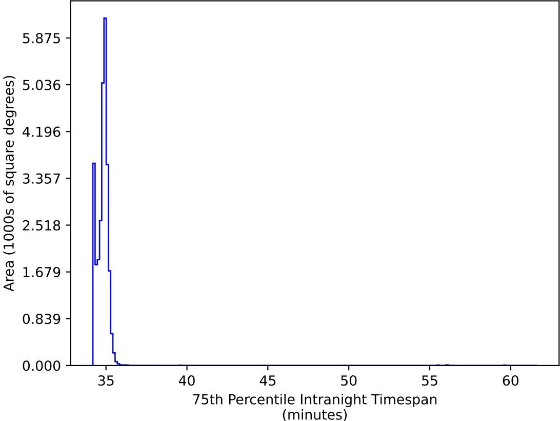
ddf_acor_sf10_lsf20_lsr20_v3.4_10yrs All sky: 75th Percentile Intranight Timespan
