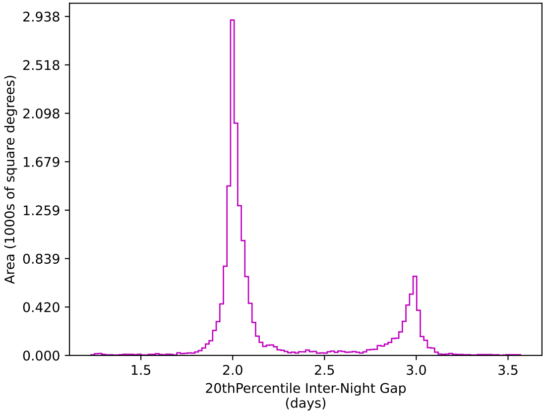
ddf_acor_sf10_lsf20_lsr20_v3.4_10yrs WFD z band: 20thPercentile Inter-Night Gap
