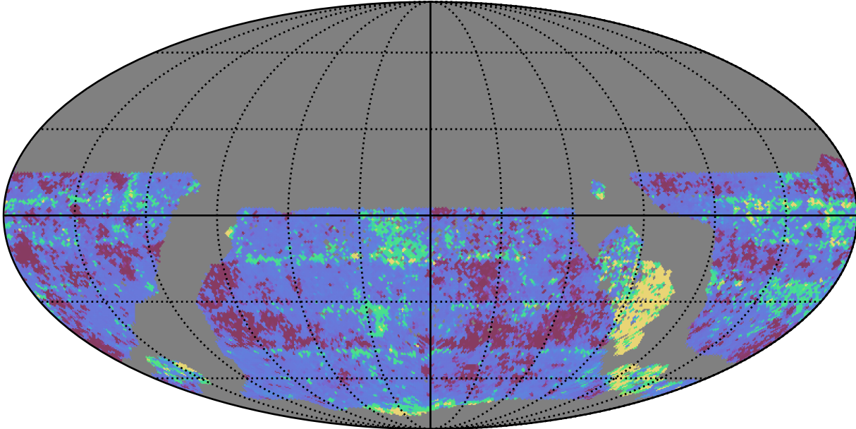
ddf_acor_sf10_lsf20_lsr20_v3.4_10yrs WFD y band: 20thPercentile Inter-Night Gap
