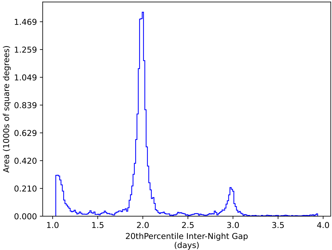
ddf_acor_sf10_lsf20_lsr20_v3.4_10yrs WFD y band: 20thPercentile Inter-Night Gap
