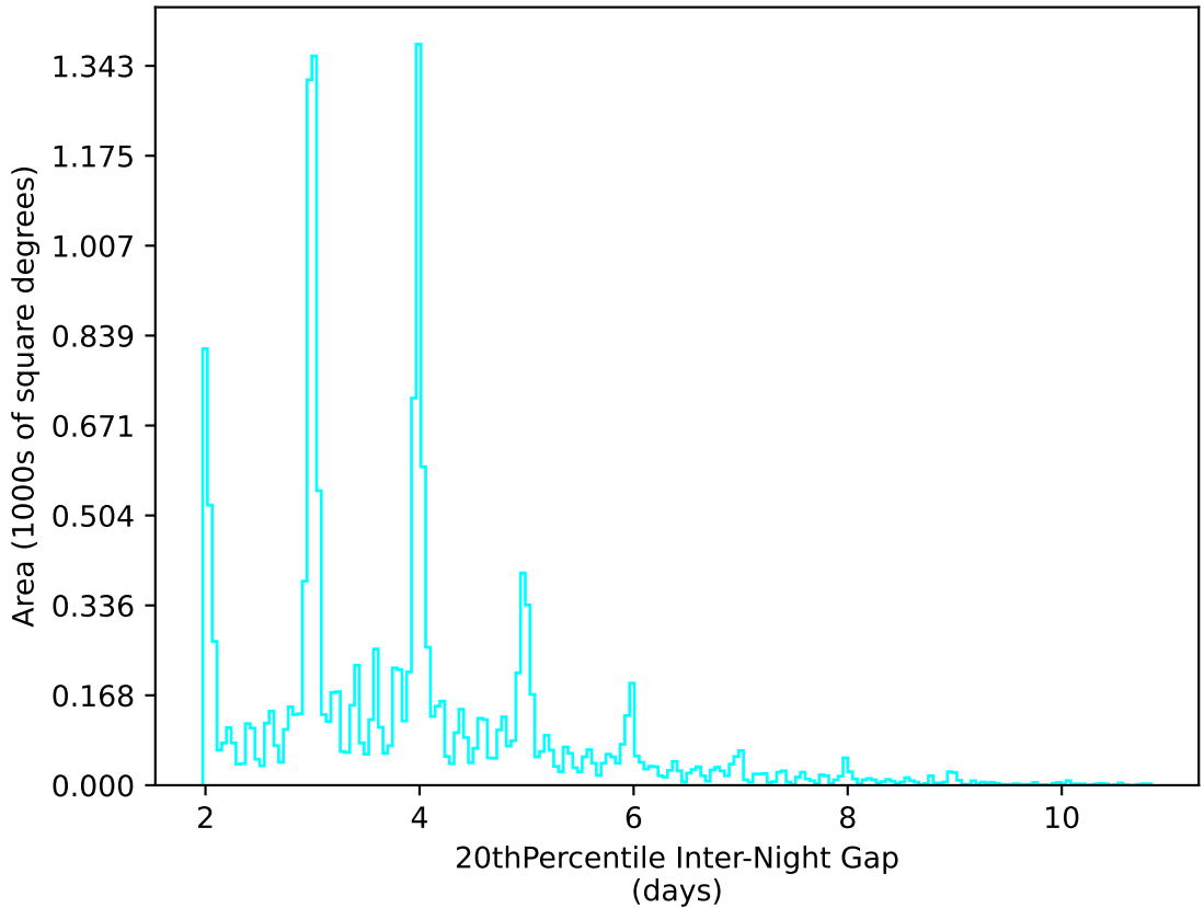
ddf_acor_sf10_ls20_lsr20_v3.4_10yrs WFD u band: 20thPercentile Inter-Night Gap
