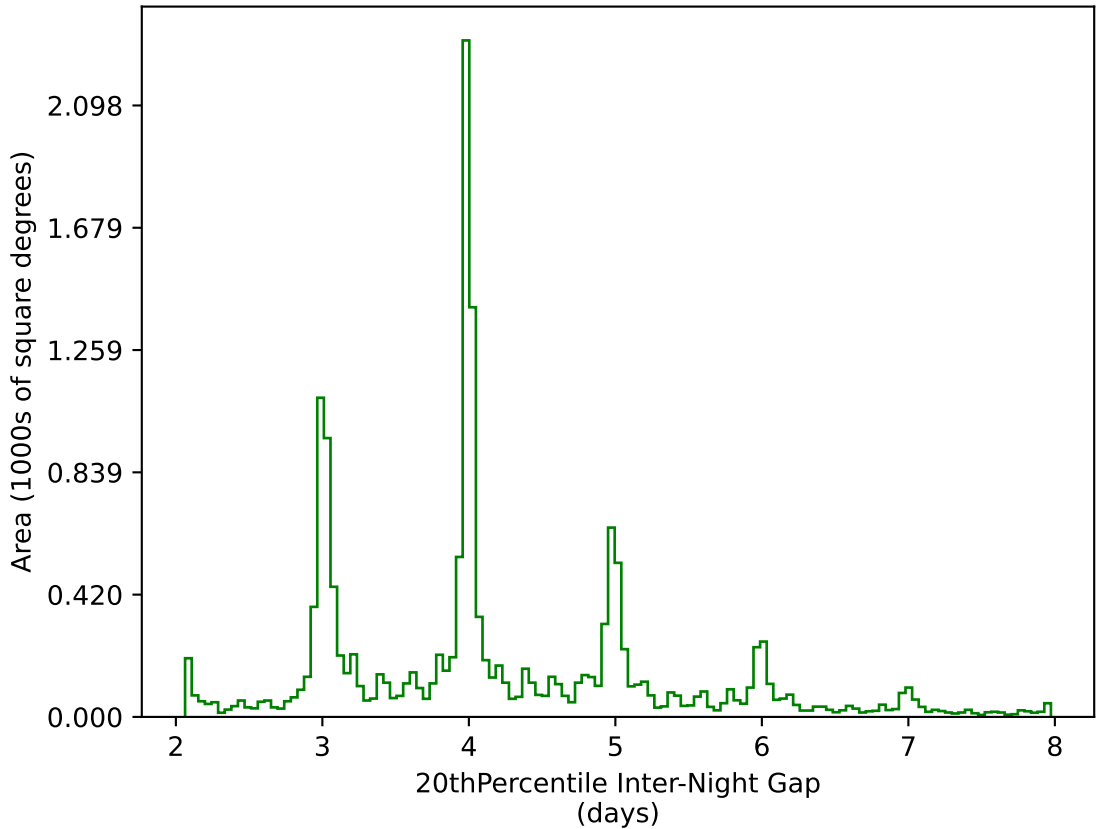
ddf_acor_sf10_lsf20_lsr20_v3.4_10yrs WFD g band: 20thPercentile Inter-Night Gap
