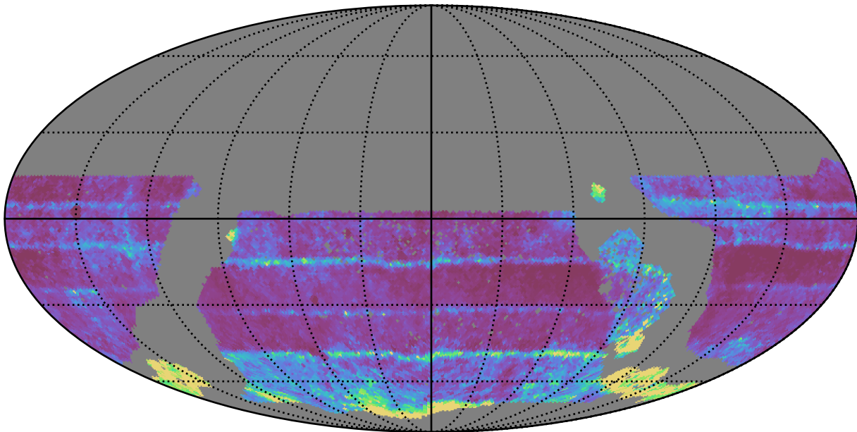
ddf_acor_sf10_lsf20_lsr20_v3.4_10yrs WFD all bands: 20thPercentile Inter-Night Gap
