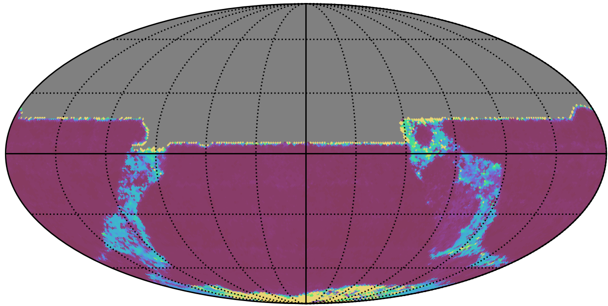
ddf_acor_sf10_lsf20_lsr20_v3.4_10yrs All sky y band: 20thPercentile Inter-Night Gap
