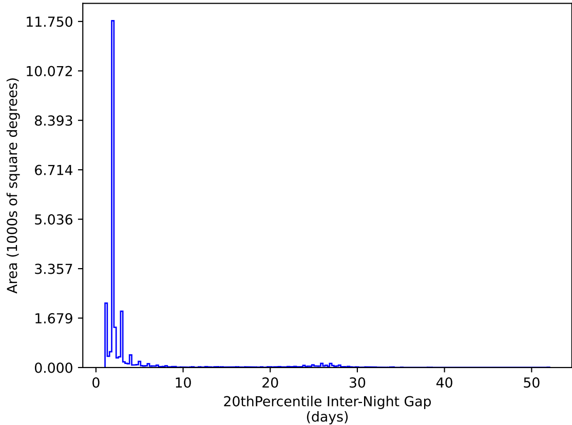
ddf_acor_sf10_lsf20_lsr20_v3.4_10yrs All sky y band: 20thPercentile Inter-Night Gap
