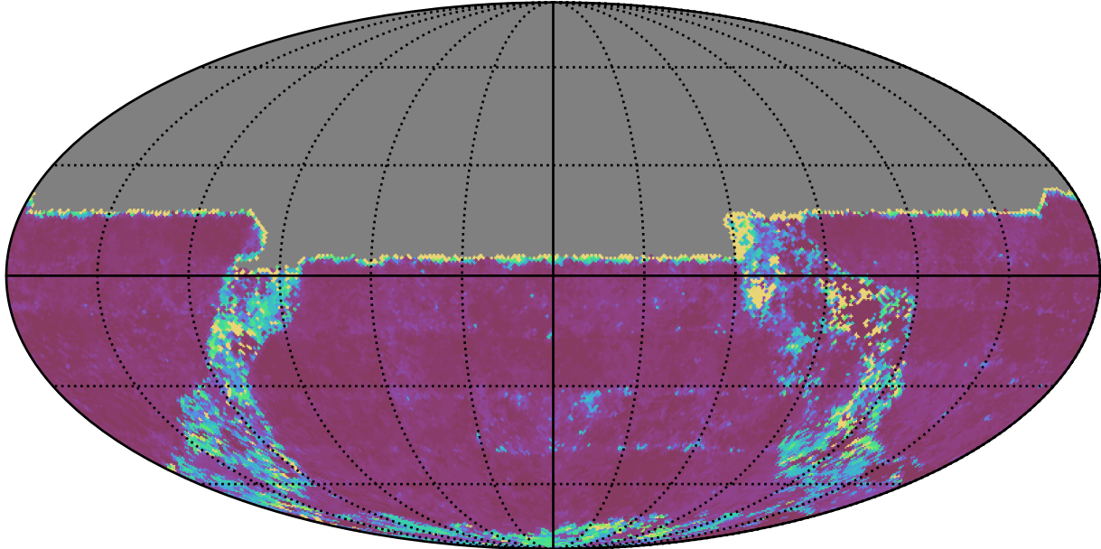
ddf_acor_sf10_lsf20_lsr20_v3.4_10yrs All sky u band: 20thPercentile Inter-Night Gap
