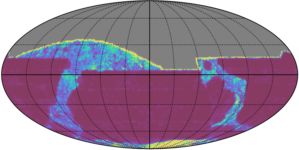
ddf_acor_sf10_lsf20_lsr20_v3.4_10yrs All sky i band: 20thPercentile Inter-Night Gap
