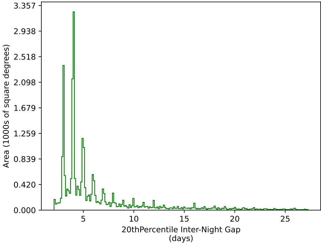
ddf_acor_sf10_ls20_lsr20_v3.4_10yrs All sky g band: 20thPercentile Inter-Night Gap
