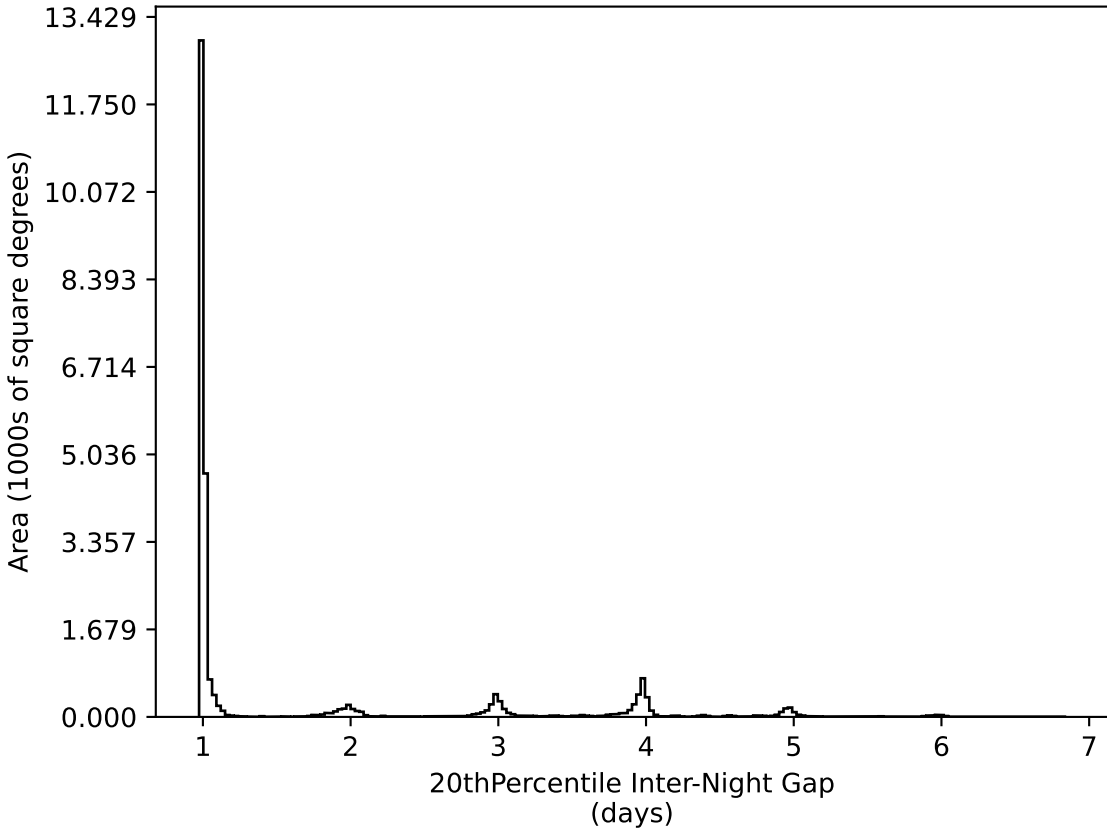
ddf_acor_sf10_lsf20_lsr20_v3.4_10yrs All sky all bands: 20thPercentile Inter-Night Gap
