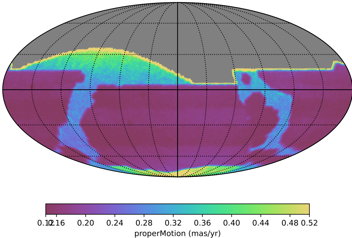
ddf_acor_sf10_lsf20_lsr20_v3.4_10yrs : properMotion
