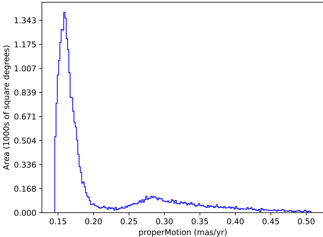
ddf_acor_sf10_lsf20_lsr20_v3.4_10yrs : properMotion
