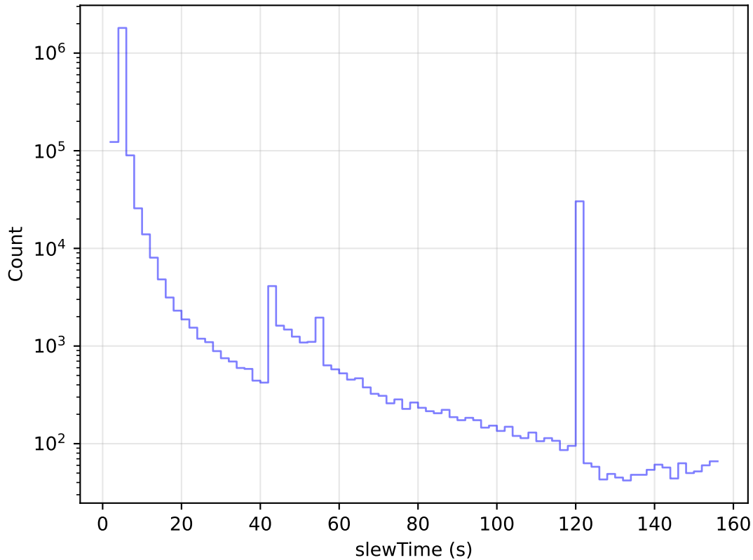
ddf_acor_sf10_lsf20_lsr20_v3.4_10yrs All visits: Slew Time Histogram
