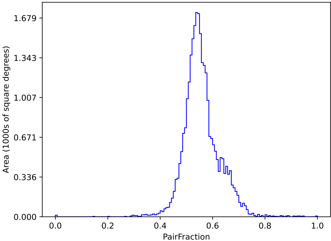
ddf_acor_sf10_lsf20_lsr20_v3.4_10yrs (g or r or i): PairFraction
