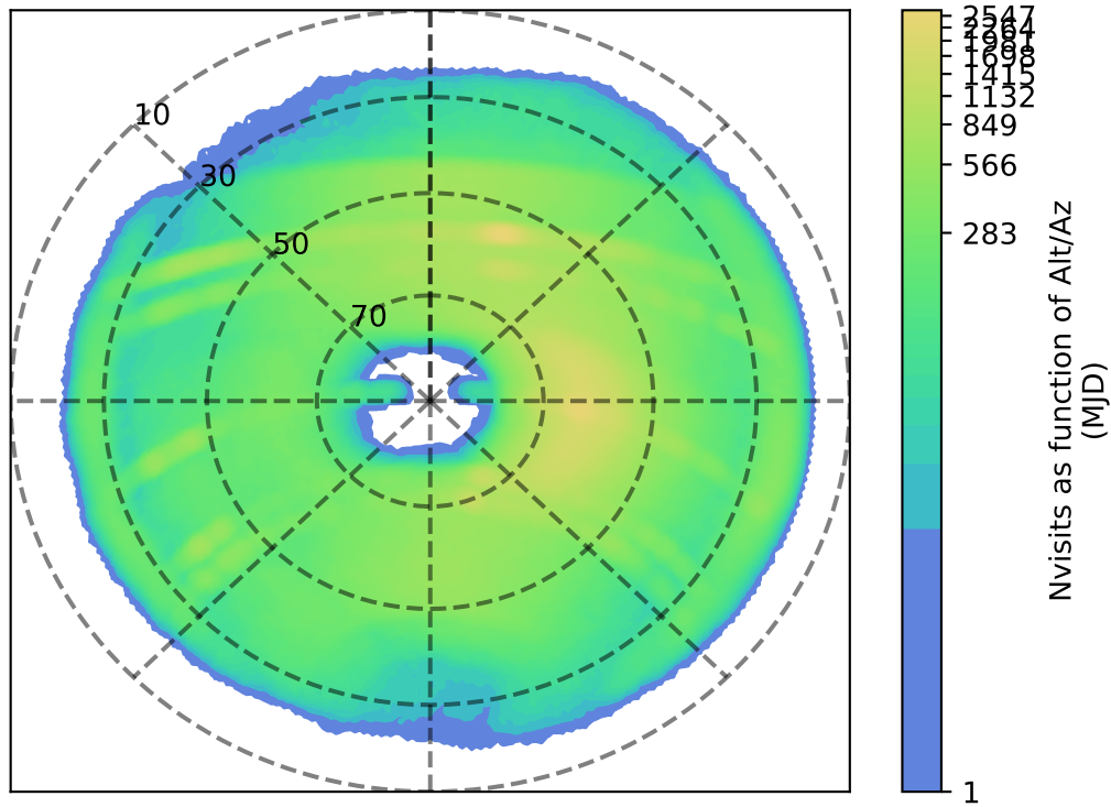
ddf_acor_sf10_lsf20_lsr20_v3.4_10yrs z: Nvisits as function of Alt/Az
