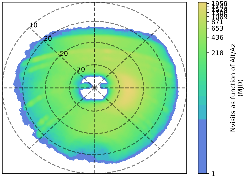
ddf_acor_sf10_lsf20_lsr20_v3.4_10yrs y: Nvisits as function of Alt/Az
