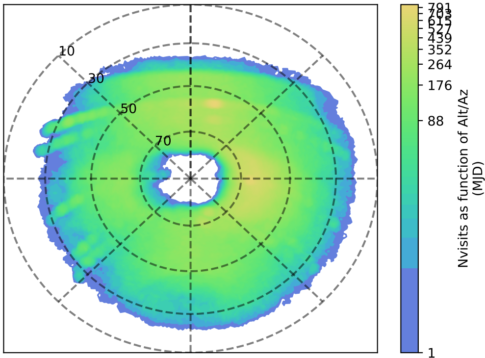
ddf_acor_sf10_lsf20_lsr20_v3.4_10yrs u: Nvisits as function of Alt/Az
