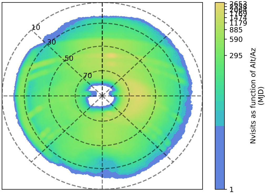
ddf_acor_sf10_lsf20_lsr20_v3.4_10yrs r: Nvisits as function of Alt/Az
