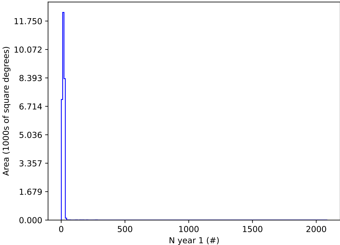
ddf_acor_sf10_lsf20_lsr20_v3.4_10yrs i and night < 365: N year 1
