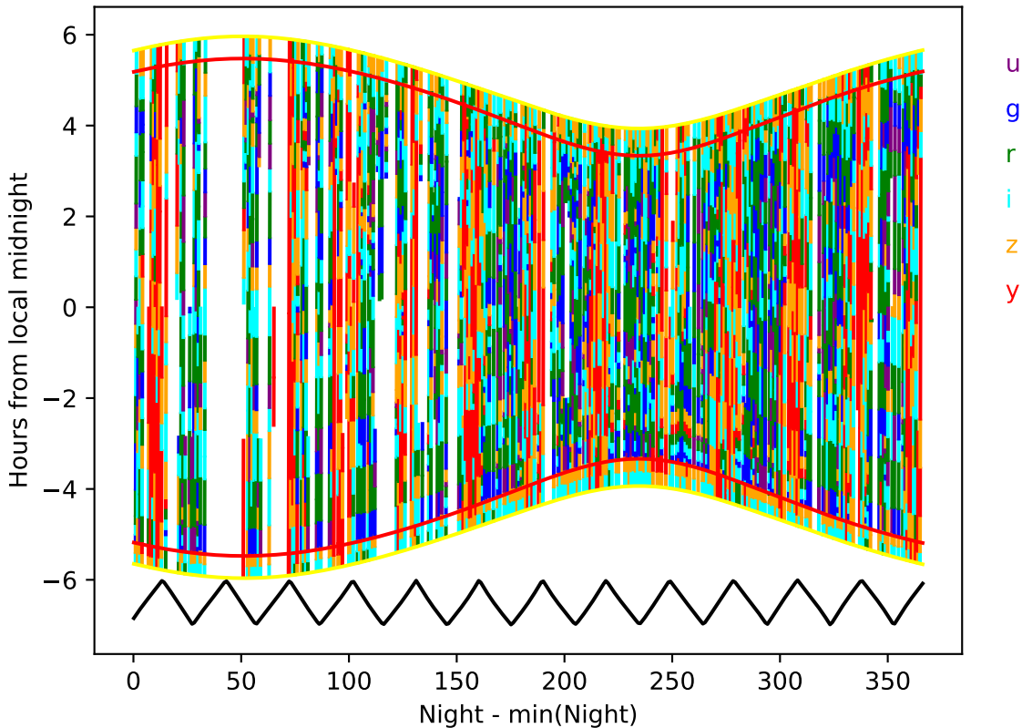
ddf_acor_sf10_lsf20_lsr20_v3.4_10yrs year 8-9: Hourglass
