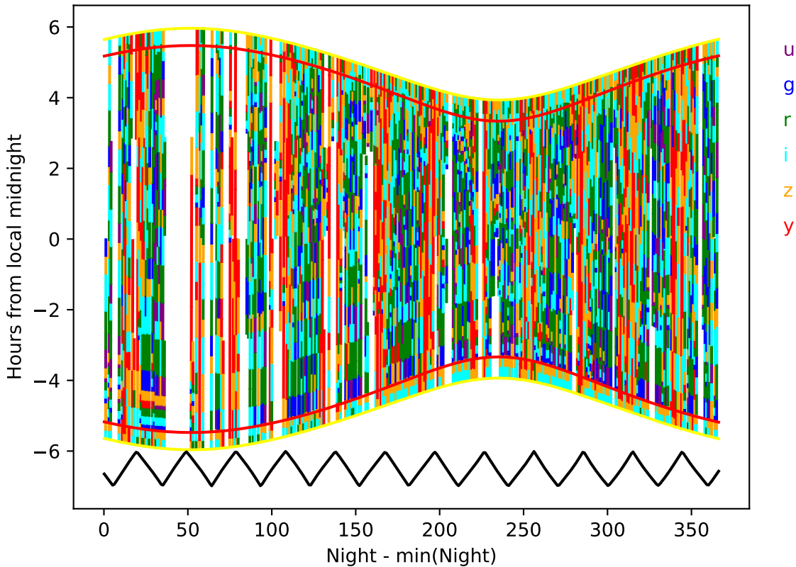
ddf_acor_sf10_lsf20_lsr20_v3.4_10yrs year 2-3: Hourglass
