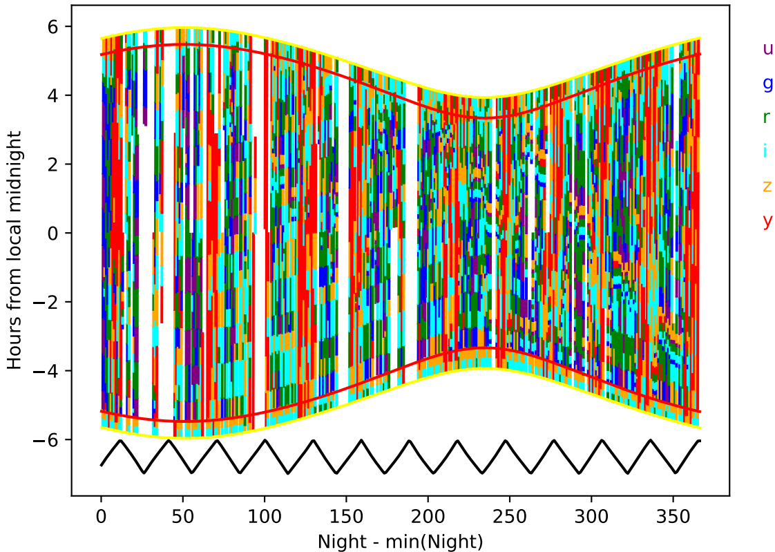
ddf_acor_sf10_lsf20_lsr20_v3.4_10yrs year 0-1: Hourglass
