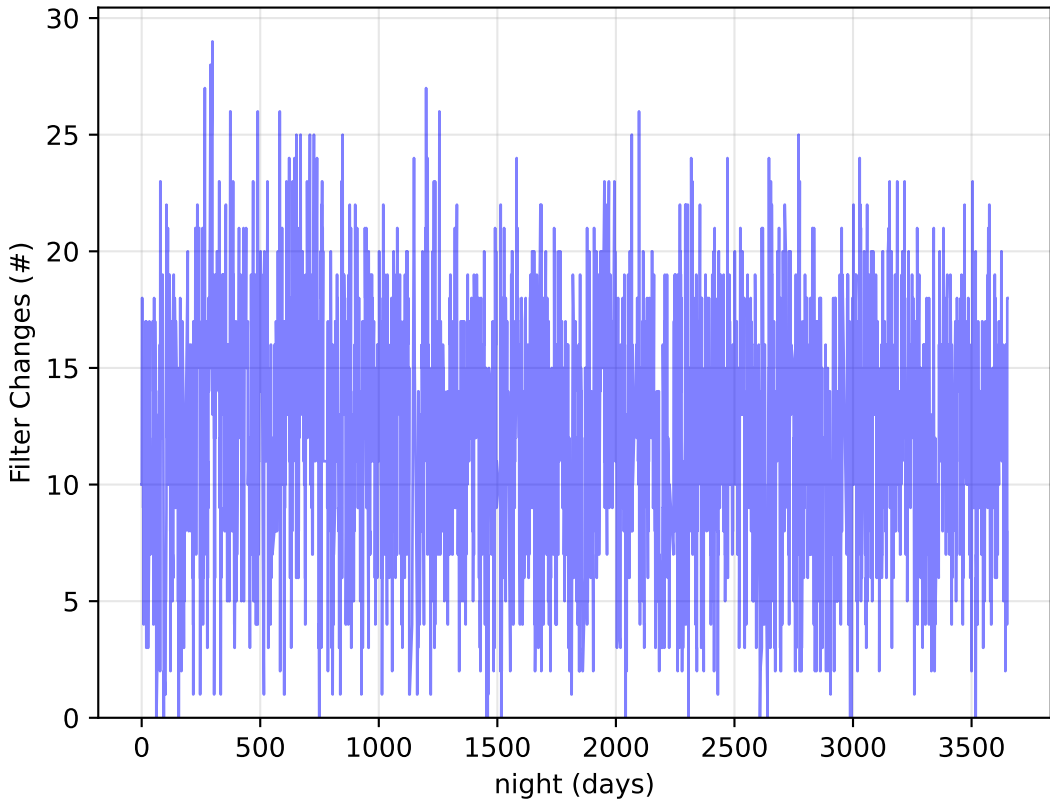
ddf_acor_sf10_lsf20_lsr20_v3.4_10yrs : Filter Changes
