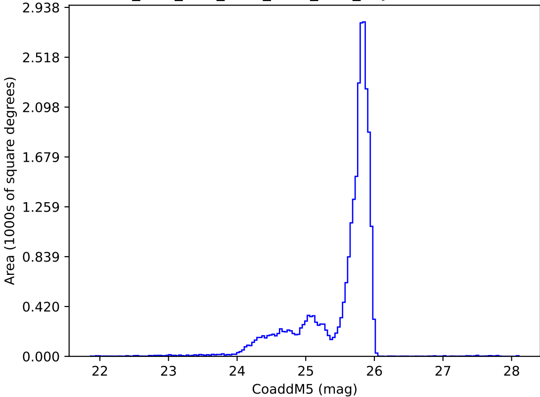
ddf_acor_sf10_lsf20_lsr20_v3.4_10yrs z: CoaddM5
