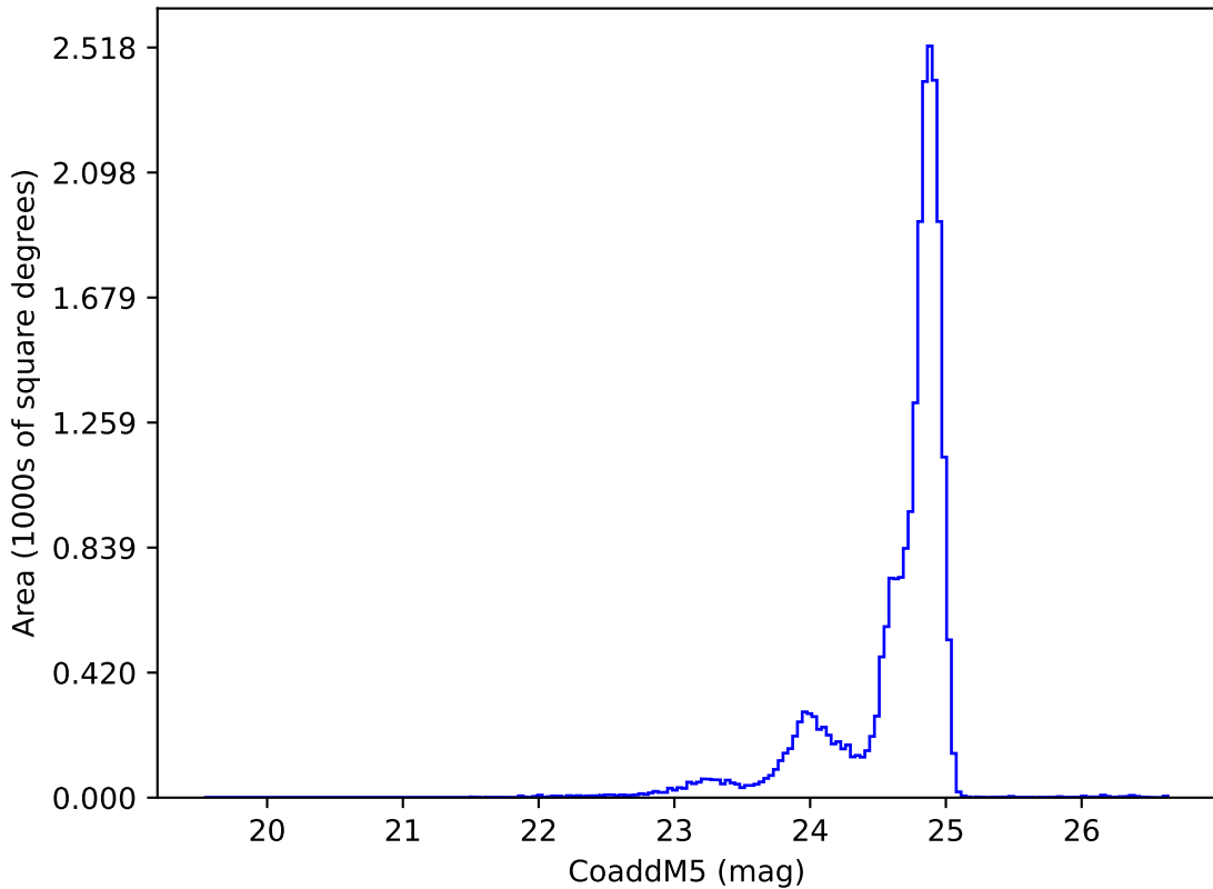
ddf_acor_sf10_lsf20_lsr20_v3.4_10yrs y: CoaddM5
