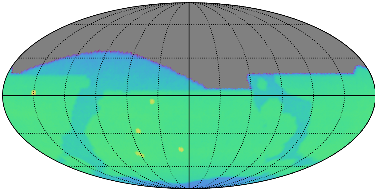
ddf_acor_sf10_lsf20_lsr20_v3.4_10yrs i: CoaddM5
