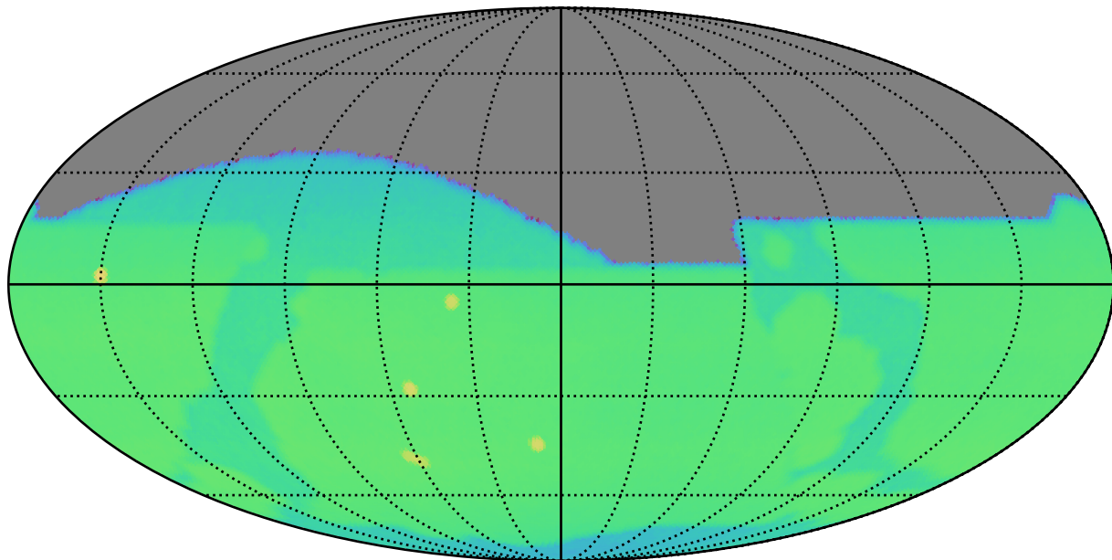
ddf_acor_sf10_lsf20_lsr20_v3.4_10yrs : CoaddM5
