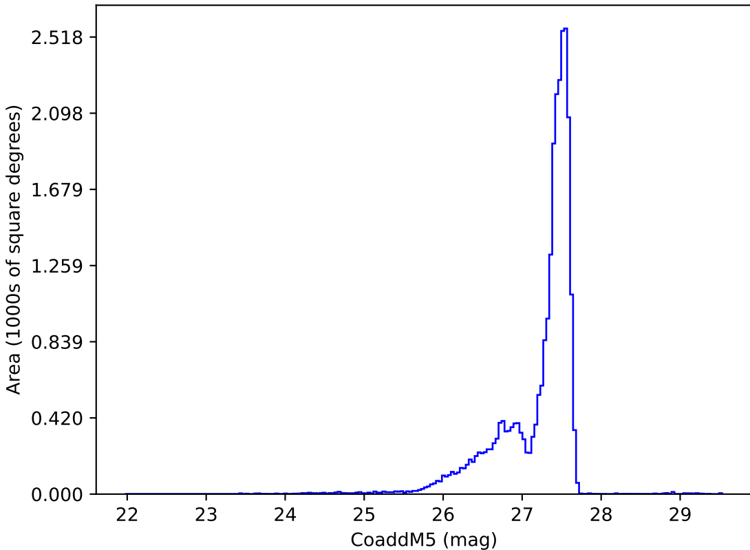
ddf_acor_sf10_lsf20_lsr20_v3.4_10yrs : CoaddM5
