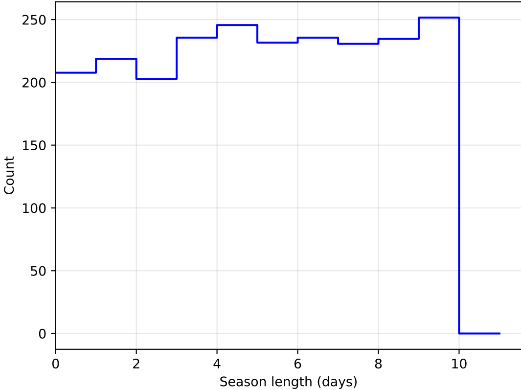
ddf_acor_sf10_lsf20_lsr20_v3.4_10yrs DD:XMM_LSS all bands: SeasonLength
