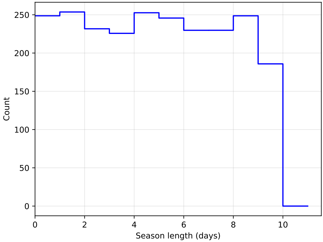
ddf_acor_sf10_lsf20_lsr20_v3.4_10yrs DD:ECDFS all bands: SeasonLength
