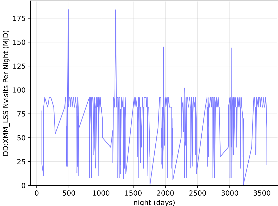
ddf_acor_sf10_lsf20_lsr20_v3.4_10yrs all bands: DD:XMM_LSS Nvisits Per Night
