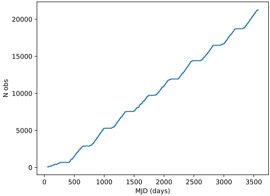
ddf_acor_sf10_lsf20_lsr20_v3.4_10yrs all bands: DD:ELAISS1 Cumulative NVisits
