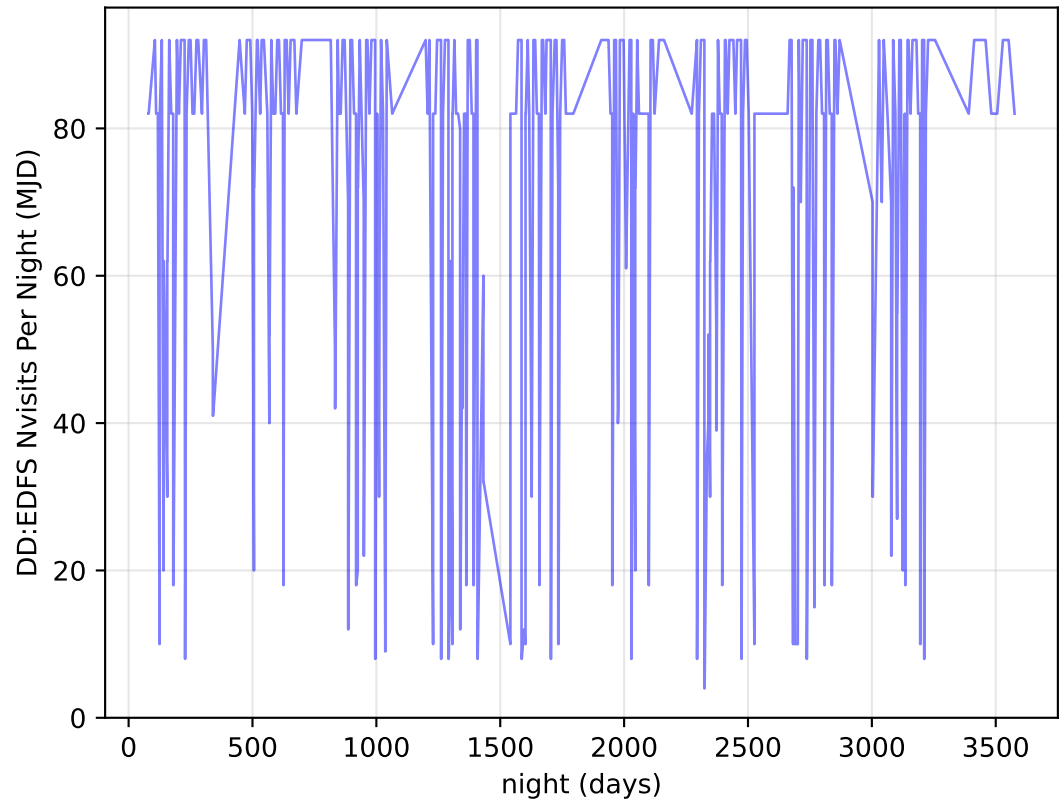
ddf_acor_sf10_lsf20_lsr20_v3.4_10yrs all bands: DD:EDFS Nvisits Per Night
