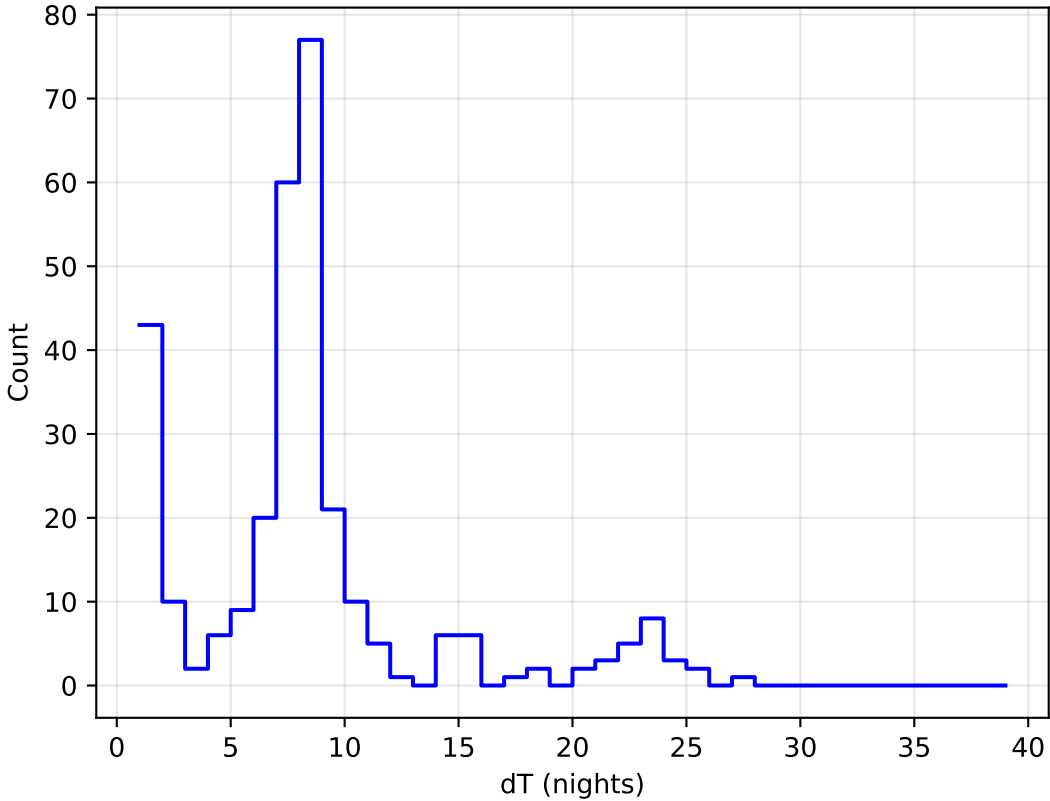
ddf_acor_sf10_lsf20_lsr20_v3.4_10yrs all bands: DD:EDFS Delta Nights Histogram
