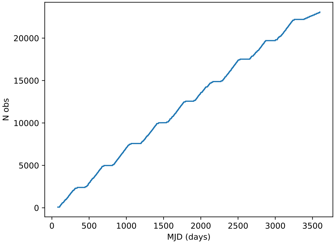
ddf_acor_sf10_lsf20_lsr20_v3.4_10yrs all bands: DD:EDFS Cumulative NVisits
